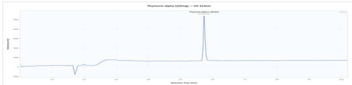
Representative chromatogram, Conformity V2 (99.61% purity, closest to batch mean of 99.58%)
